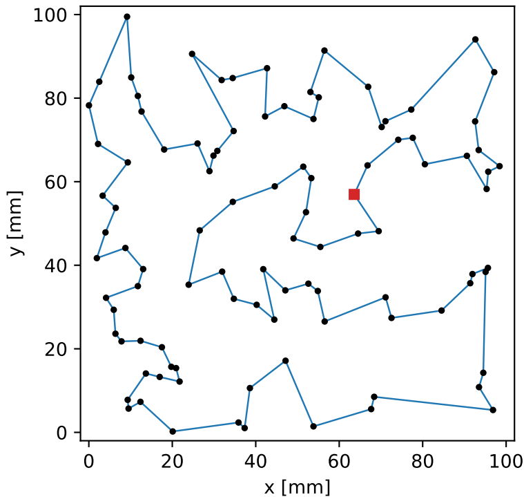
tabu search, 1 s (length 787.7)
