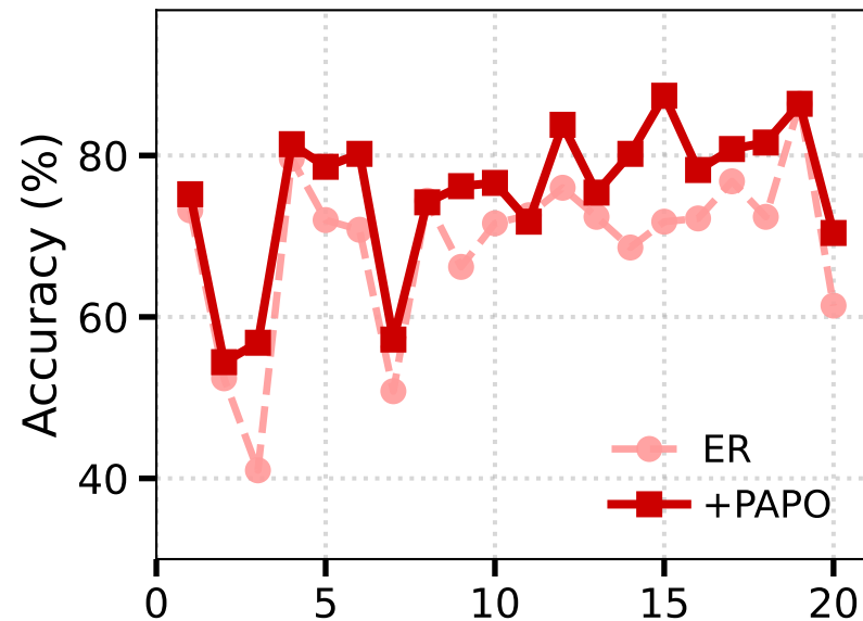
GPM
