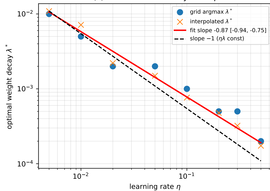
(c) \lambda^* moves inversely with \eta
