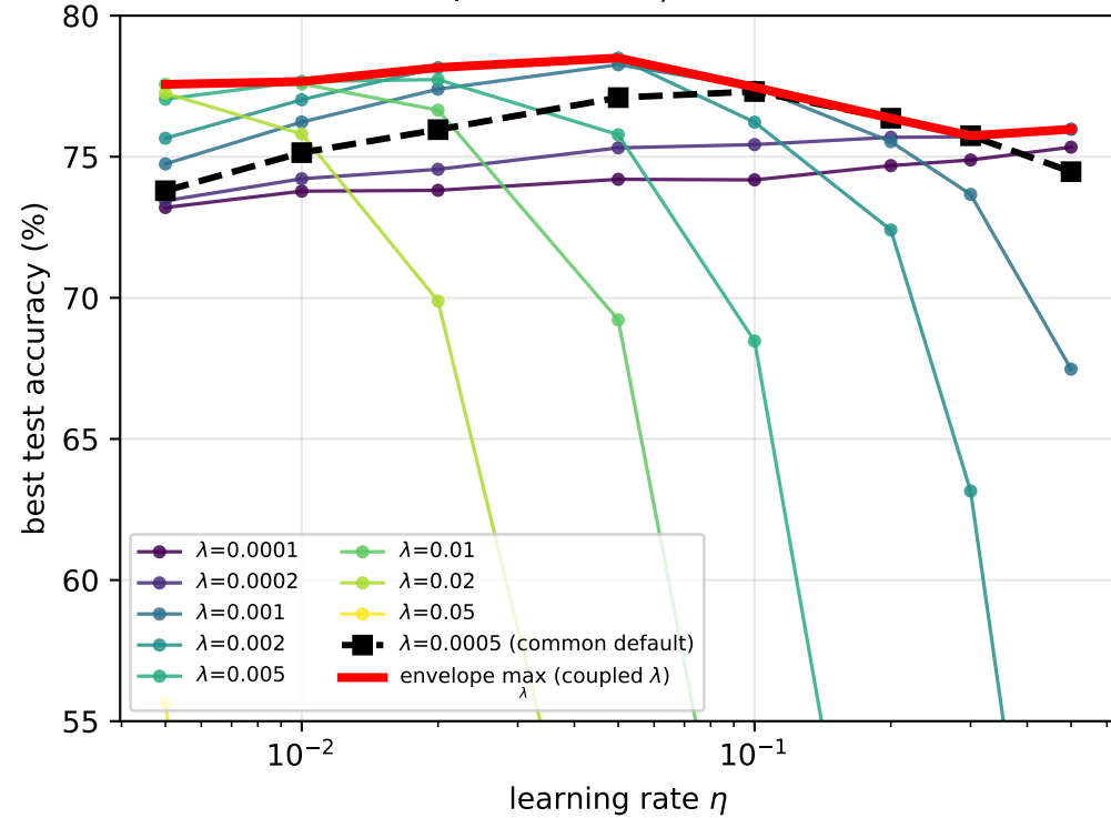
(a) No fixed \lambda reaches the envelope ResNet-18 / CIFAR-100, mean of 2 seeds
