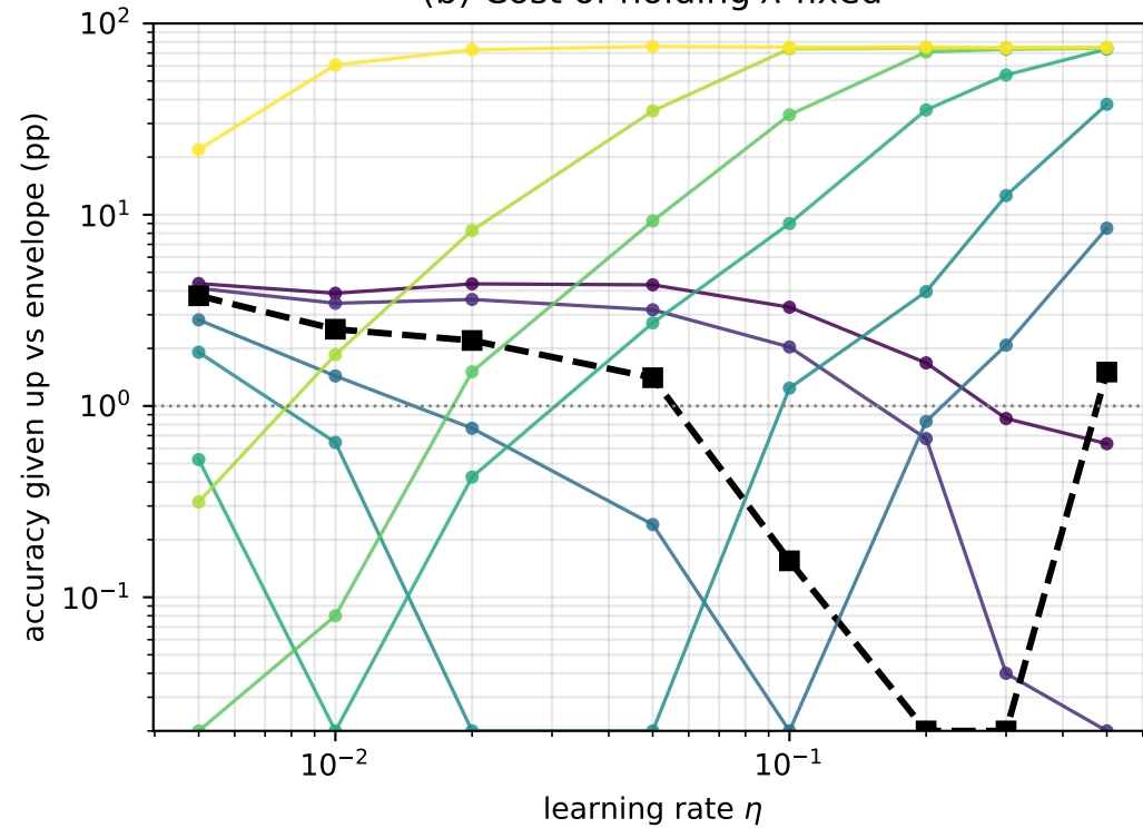
(b) Cost of holding \lambda fixed
