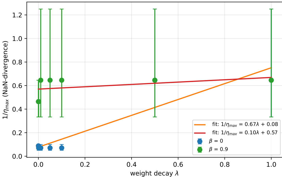
Explosion boundary against weight decay theory: 1/\eta_{max} = \lambda + L/2
