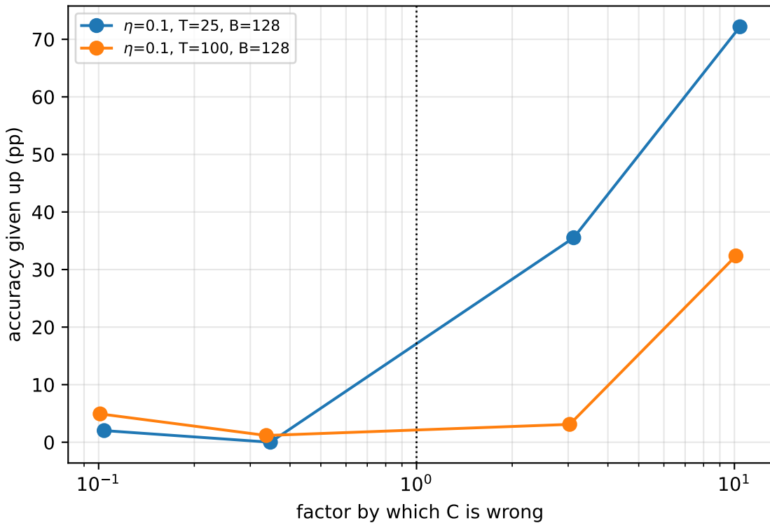
Cost of mis-specifying the constant
