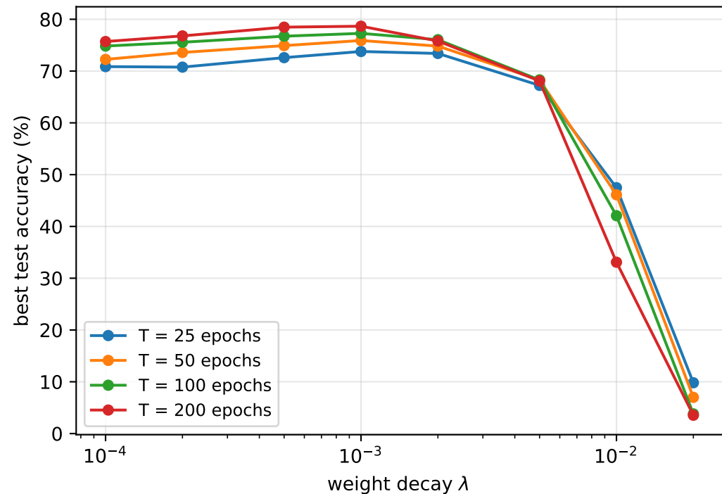
(a) Accuracy against \lambda at each training length ResNet-18 / CIFAR-100, \eta = 0.1 , B = 128
