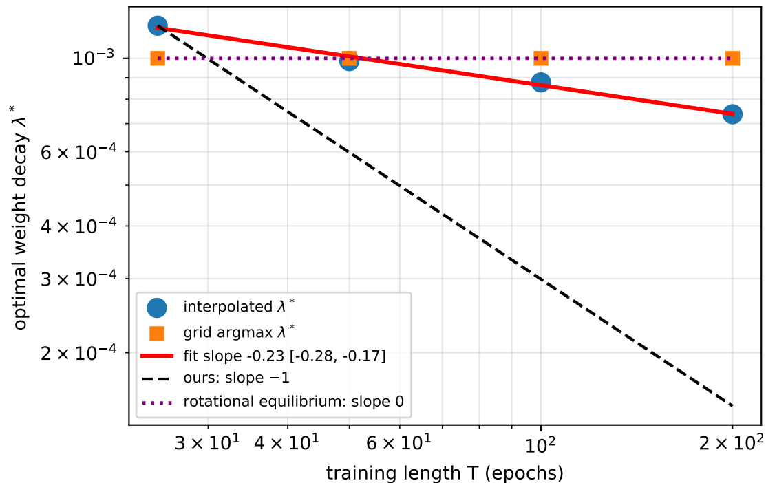
(b) \lambda^* against T : the discriminating test (negative for slope -1 )
