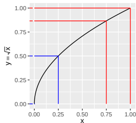
Transformation: g(x) = \sqrt{x}
