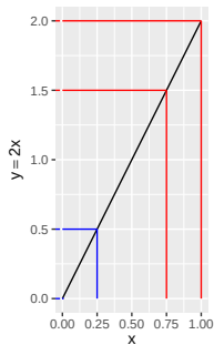
Transformation: g(x) = 2x
