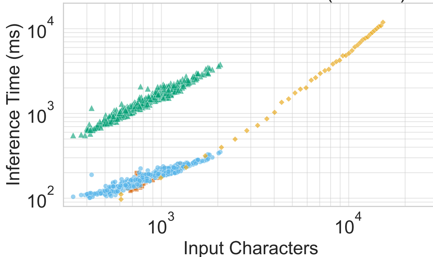
Granite on Macbook Pro (M4 Pro)
