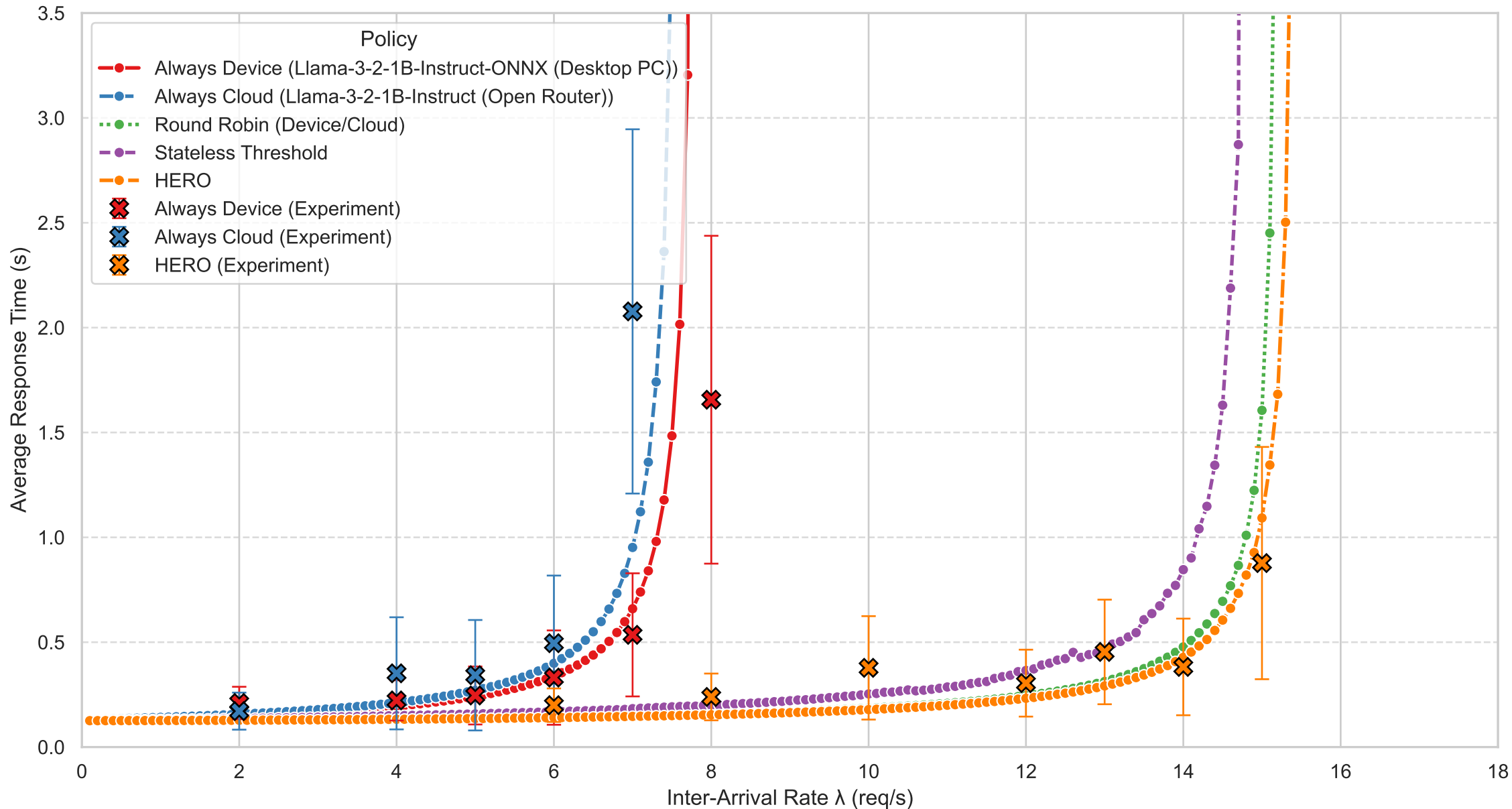
Policy Performance: Average Response Time vs. Inter-Arrival Rate ( \lambda ) on AG-News Dataset
