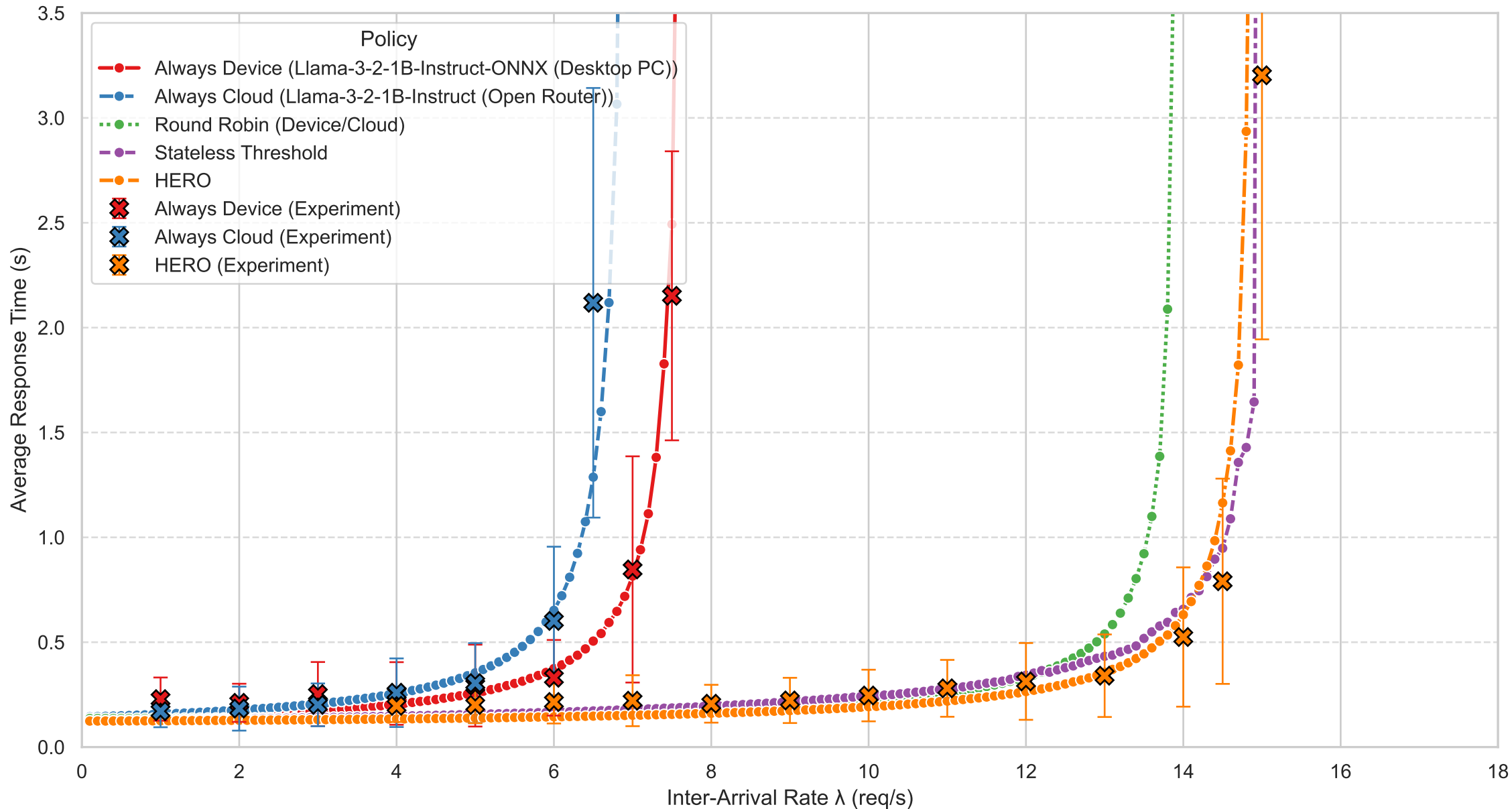
Policy Performance: Average Response Time vs. Inter-Arrival Rate ( \lambda ) on BoolQ Dataset
