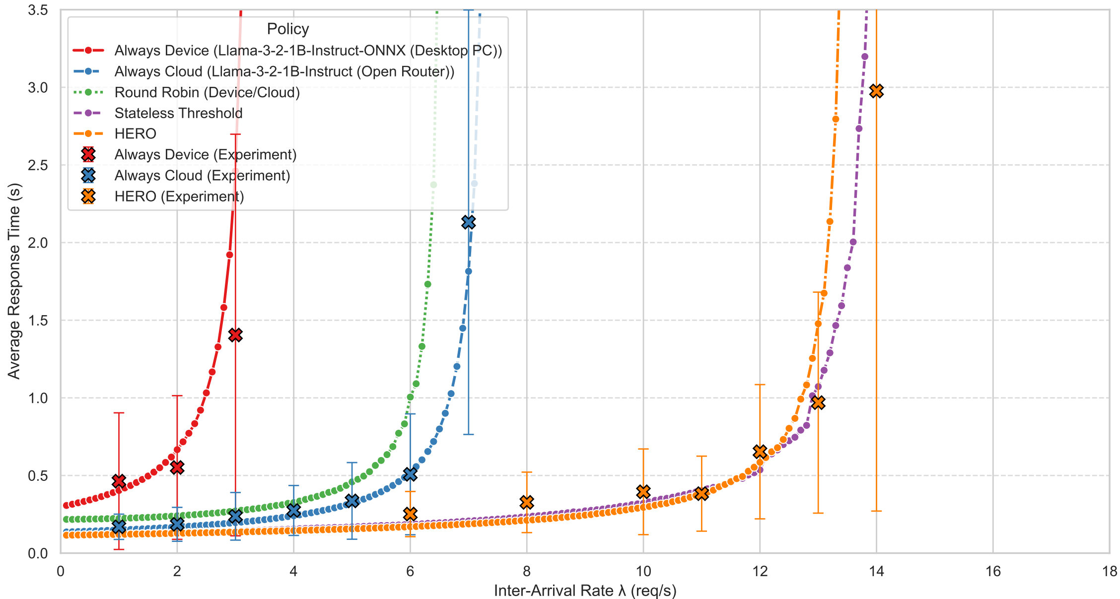
Policy Performance: Average Response Time vs. Inter-Arrival Rate ( \lambda ) on Spam/Ham Dataset
