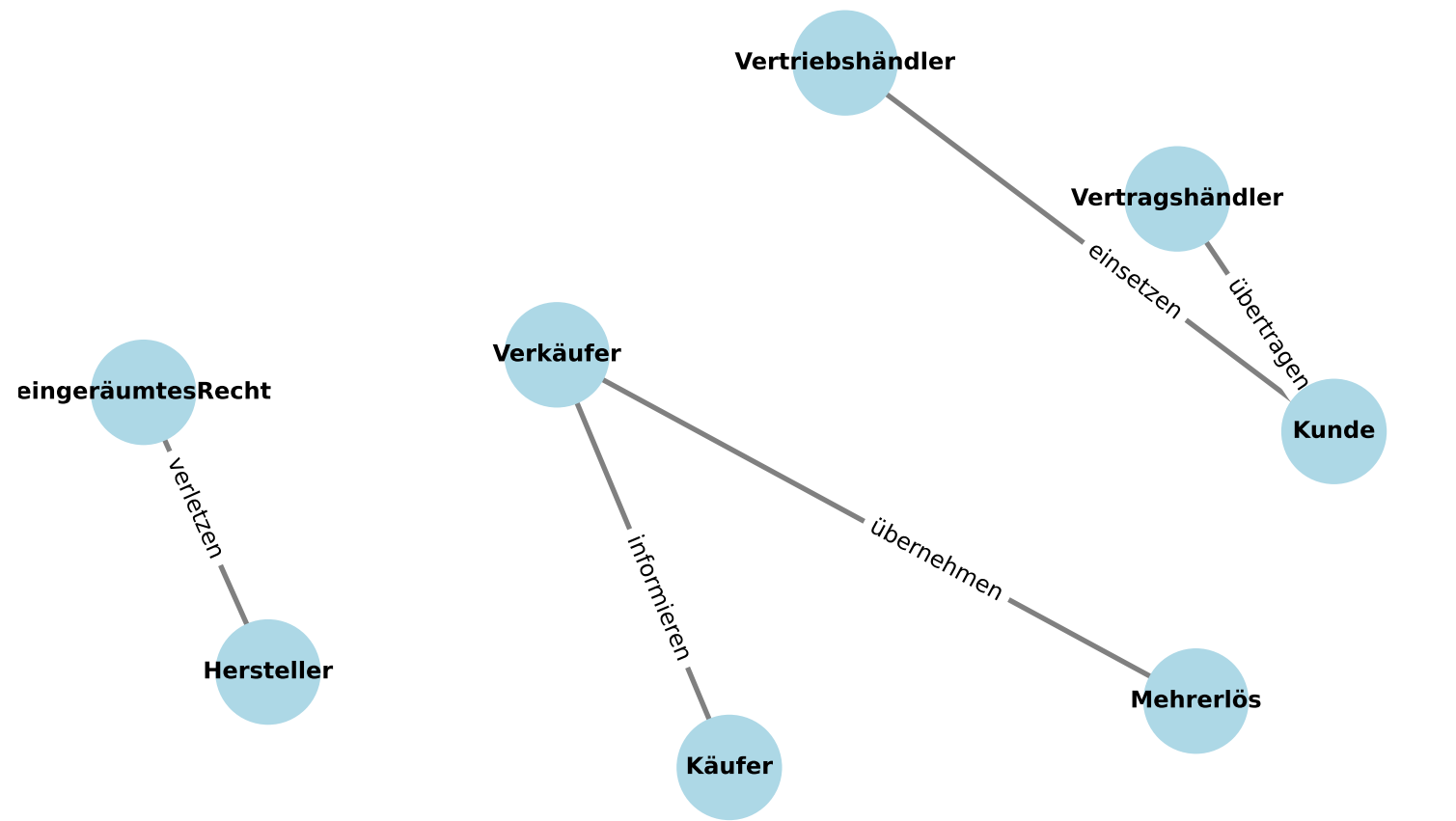
Cluster 102 - Detaillie
