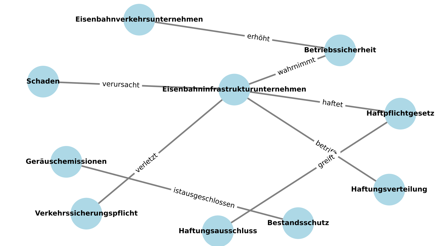
Cluster 100 - Detaillie
