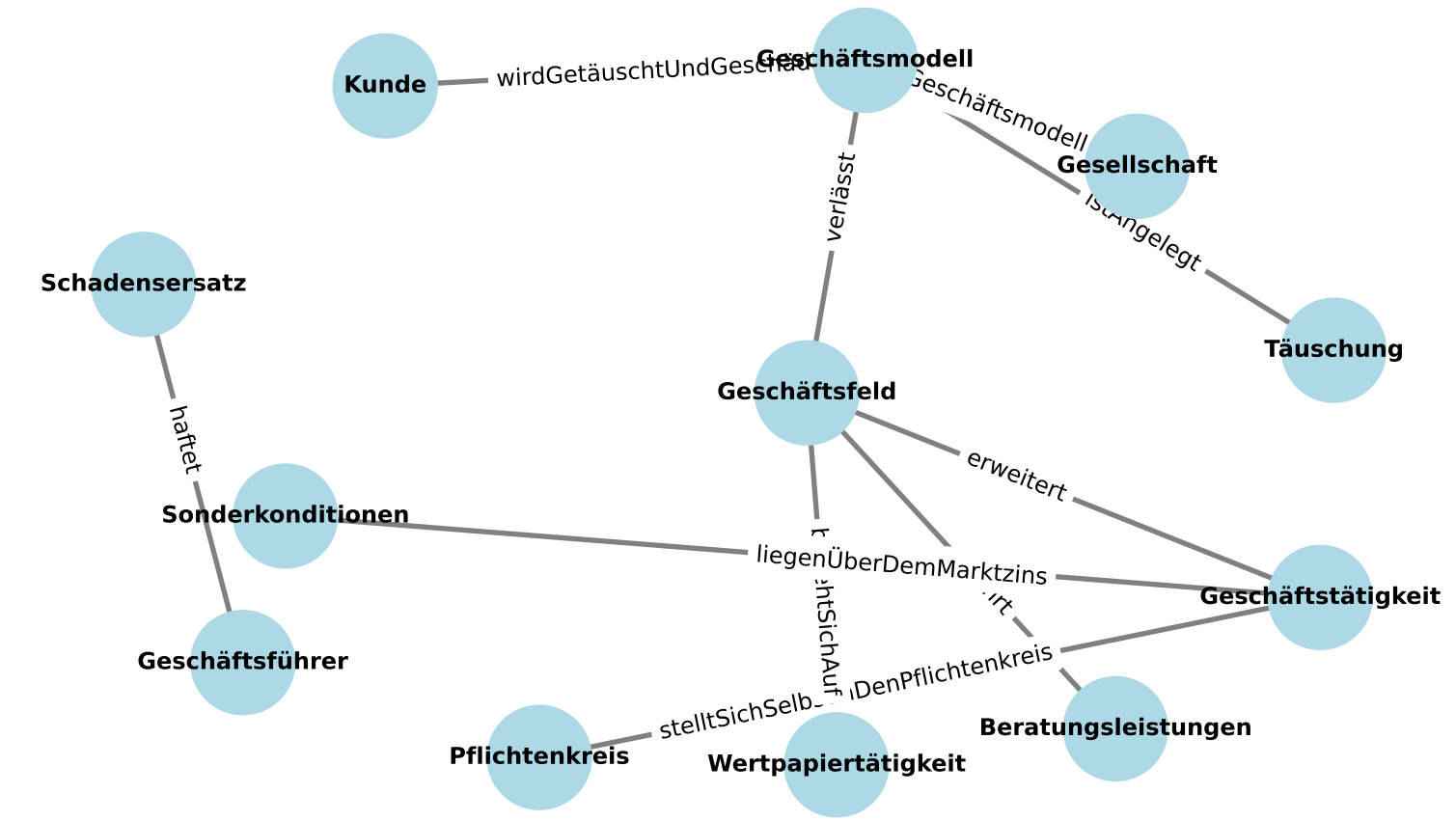
Cluster 104 - Detaillie
