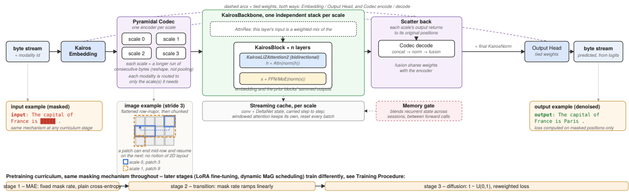
Figure 1: Kairos data and training flow, left to right. Each KairosBlock is a standard pre-norm attention+FFN residual pair; AttnRes only re-mixes what feeds into it. Training (bottom) uses one masking mechanism across three curriculum stages (MAE → transition → diffusion), illustrated with a masked-input/denoised-output example.
