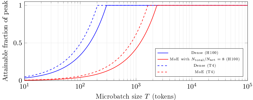
Figure 3: Model output (Eq. ??), not a measurement: the fraction of peak throughput a microbatch can reach. Sparsity moves the saturation point right by N_{\text{total}}/N_{\text{act}} = 8 .
