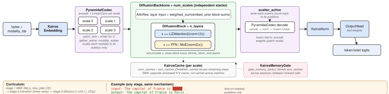
Figure 1: Kairos data and training flow, left to right. Each DiffusionBlock is a standard pre-norm attention+FFN residual pair; AttnRes only re-mixes what feeds into it. Training (bottom) uses one masking mechanism across three curriculum stages (MAE → transition → diffusion), illustrated with a masked-input/denoised-output example.
