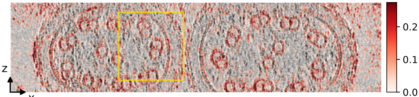
40° train
