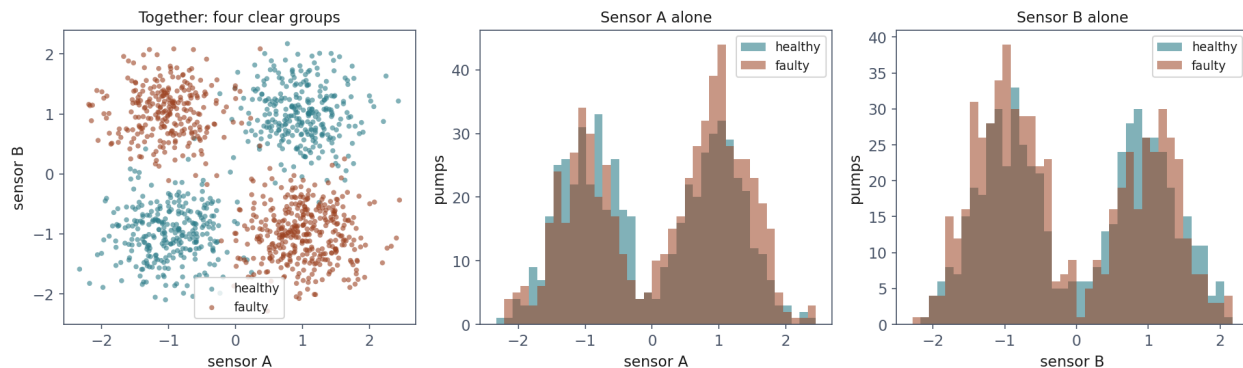
Left: together, the two sensors show four clear groups and a perfectly learnable rule. Middle and right: what Naive Bayes gets to see — each sensor alone, where the two classes sit almost exactly on top of one another.
