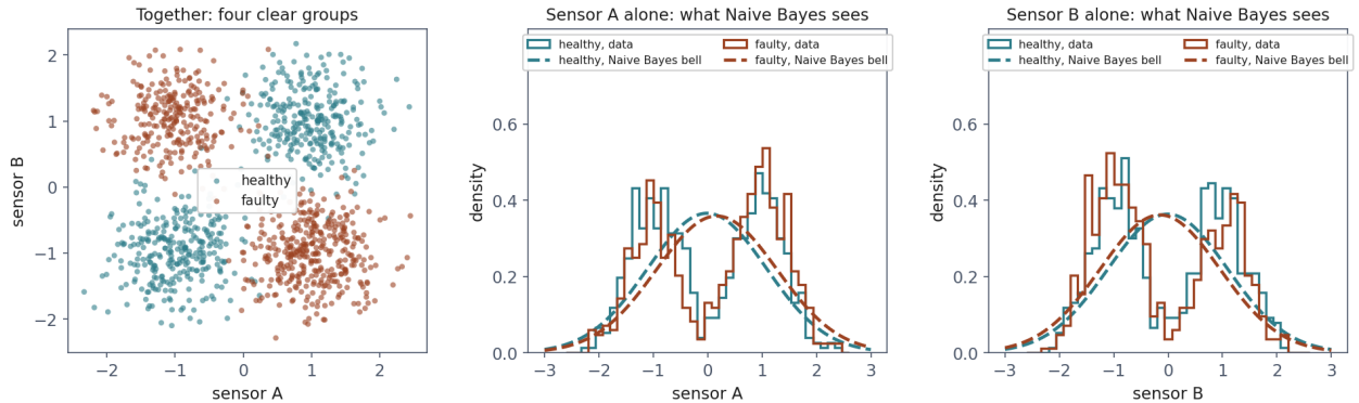
Left: together, the two sensors show four clear groups, each class owning two opposite quadrants. Middle and right: what Naive Bayes gets to see — each sensor alone. Solid outlines are the data,
