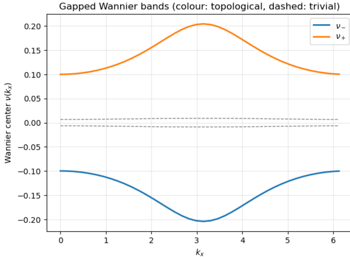
Figure 60: Wannier bands v_{\pm}(k_x) of the BBH model: gapped in the topological phase (colour), collapsed in the trivial one (dashed) - the input of the nested Wilson loop.
