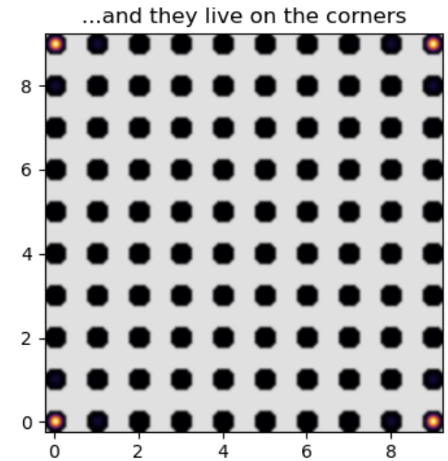
Figure 61: A finite BBH flake: four zero-energy states inside the gap (left, red) whose density sits on the four corners (right).
