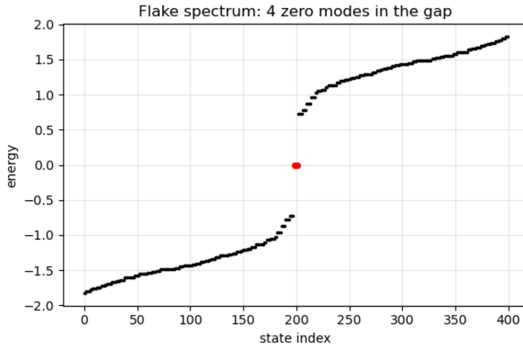
Figure 61: A finite BBH flake: four zero-energy states inside the gap (left, red) whose density sits on the four corners (right).
