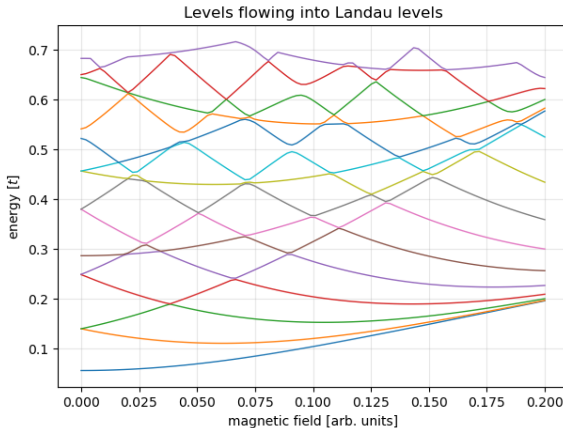
Figure 13: Spectrum of a closed disc vs magnetic field: levels condense into degenerate Landau levels (a Fock-Darwin-like fan).
