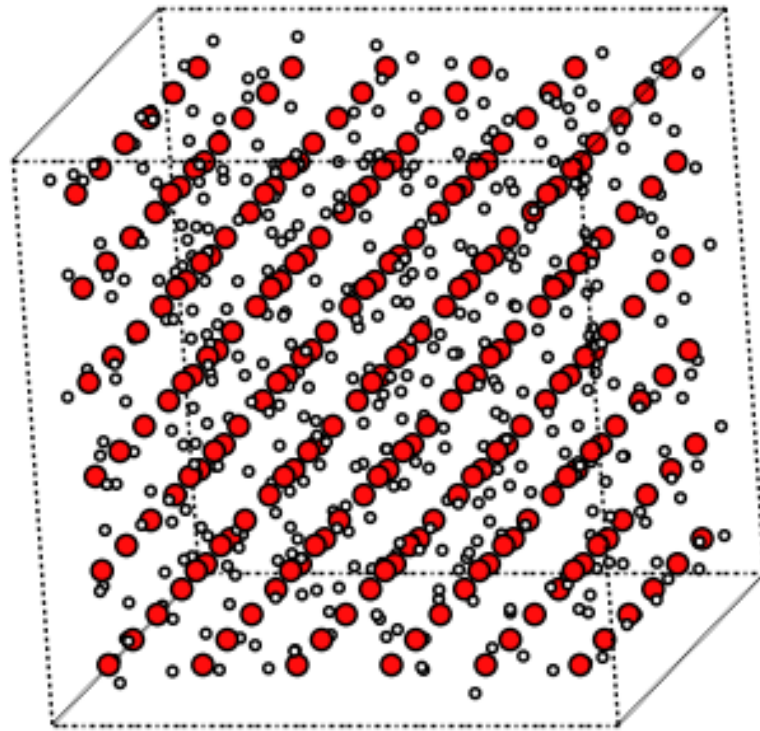
The SPC/E water box near the start of the run -- real atomic masses (15.9994, 1.008), so lammps.kitviz's own mass-to-symbol guess correctly renders oxygen and hydrogen, unlike every earlier reduced-unit chapter, which had to pick a conventional stand-in element by hand. — Figure 2 · notebook §0 · chapter 12, cell 11
