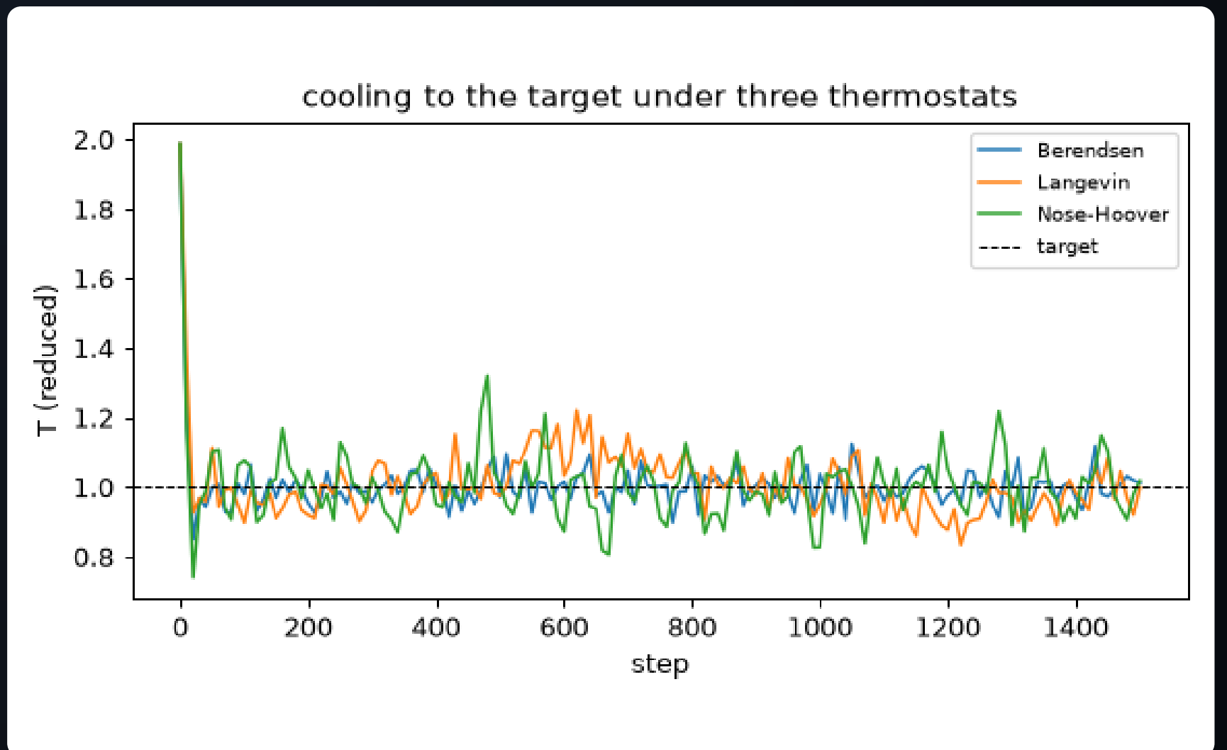
Temperature against step for the same fcc lattice, started hot ( T \sim 2 ) and cooled by three thermostats -- Berendsen, Langevin, Nose-Hoover chain -- each converging toward the target (dashed line) by its own route. — Figure 1 · notebook §0 · chapter 3, cell 4
