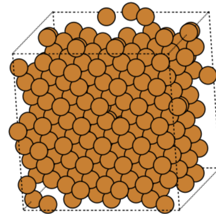
The same supercell after the vacancy is introduced and the remaining atoms are relaxed with FIRE ( f_{\text{max}} < 1e-4 ): the neighbours have relaxed inward around the missing site, visible as a locally denser region next to the gap. – Figure 2 · notebook §0 · chapter 5, cell 13
