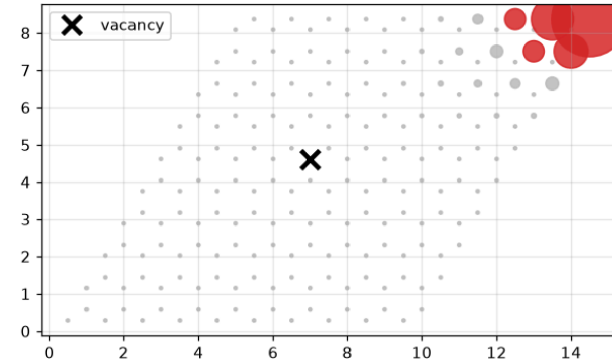
vacancy zero mode, E = +2.04e-16 — lives on the opposite sublattice
