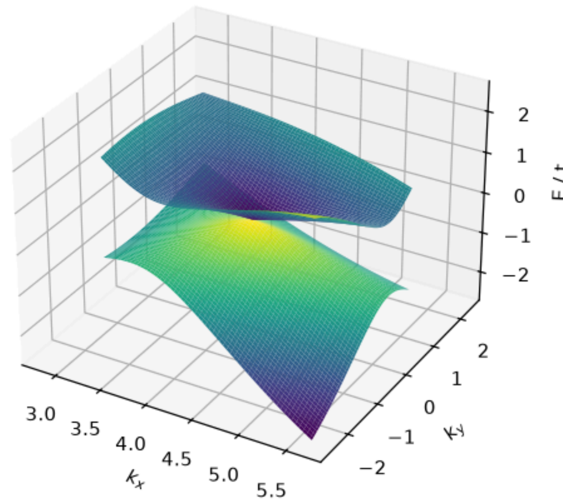
the Dirac cone at K (and its partner at K' )
