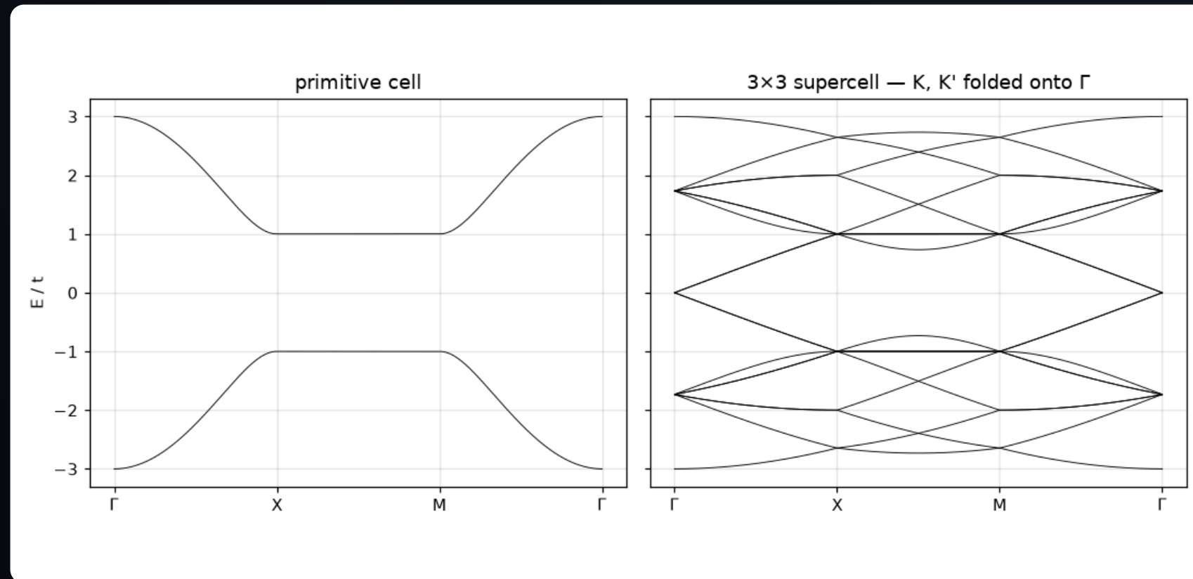
Band folding: the same graphene crystal described in its primitive cell (left) and in a 3 \times 3 supercell (right). Nothing physical changed — the supercell BZ is 9 \times smaller, so the bands fold back 9 \times denser, and both Dirac points land on \Gamma . Folding is the price of any supercell treatment (defects, disorder, magnetic flux) and must not be mistaken for new physics. — Figure 19 · notebook §7 · cell 28
