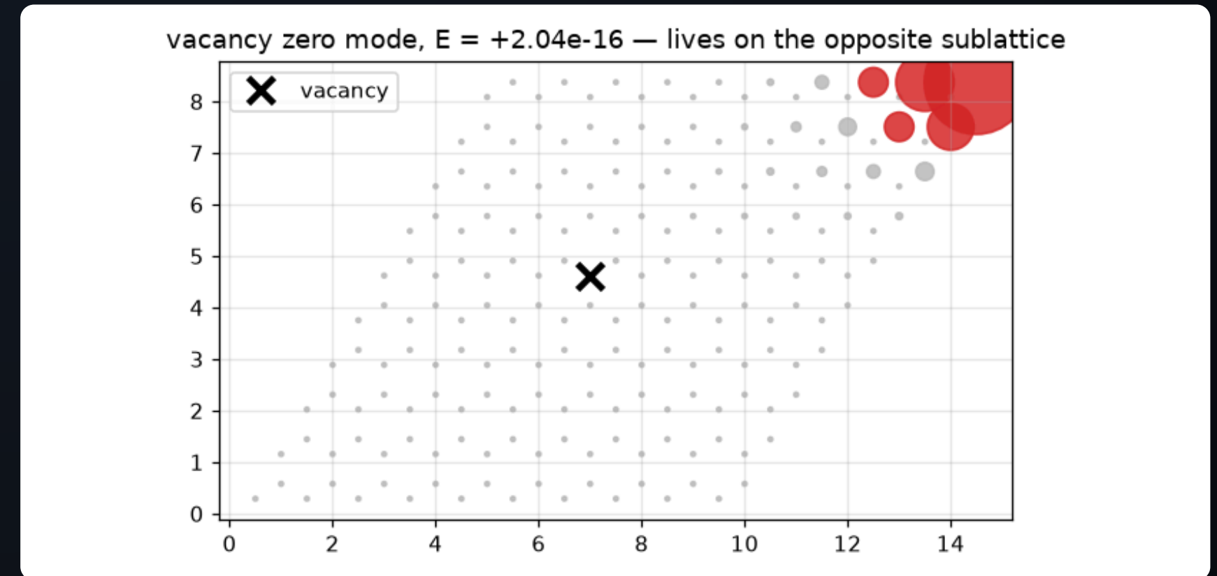
A single vacancy in a graphene flake (black cross) and the zero mode it creates (red, symbol size \propto |\psi|^2 ). Removing one A-site leaves the B sublattice with one extra site, and on any bipartite lattice that imbalance guarantees an exact E = 0 state confined to the majority sublattice — decaying as a power law around the missing atom. The proof is counting, not perturbation theory, so the mode survives at any hopping strength. — Figure 20 · notebook §7 · cell 29
