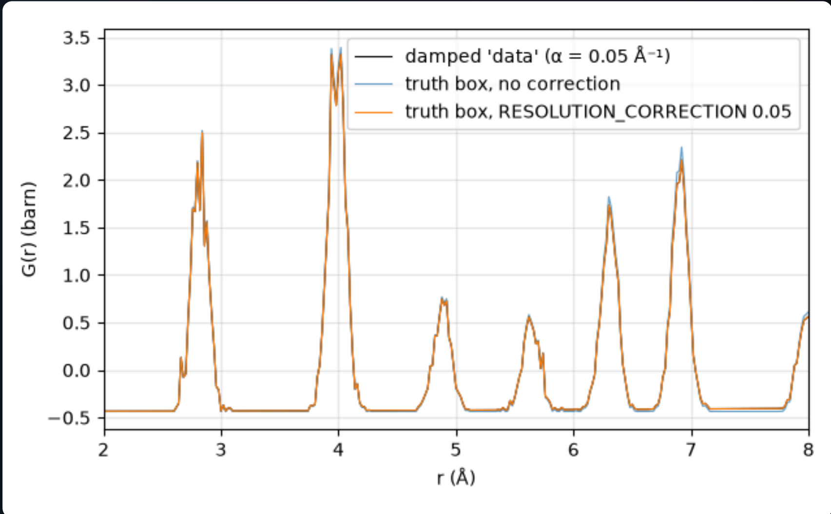
Synthetic G(r) damped by \exp(-(0.05 r)^2/2) against RMCProfile's calculated G(r) of the truth box without and with the matching RESOLUTION_CORRECTION: the corrected model's peaks shrink with r the way the data's do. — Figure 18 · notebook §29 · chapter 7, cell 7
