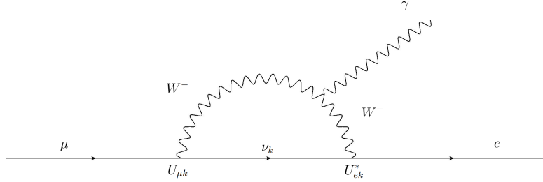
Figure 2: One-loop diagram contributing to \mu \rightarrow e\gamma in the SM.
