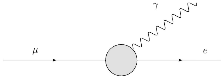
Figure 1: General amplitude for \mu \rightarrow e\gamma , with the blob representing all possible contributions.
