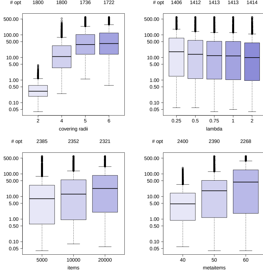
Figure 5: Computing times (in logarithmic scale) of OA+BC+f for the k-card instances aggregated by: (i) the covering radius \hat{R} , (ii) the risk-tolerance \lambda , (iii) the number of items n , and (iv) the number of metaitems \hat{n} . The number of instances solved within the time limit of 600 secs is reported above each boxplot.
