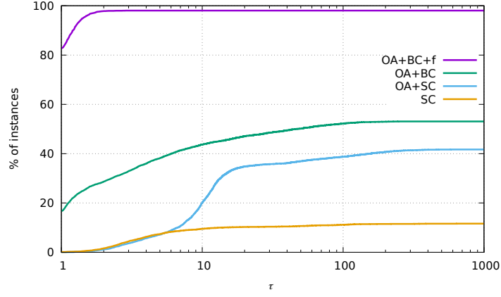
Figure 7: Performance profile comparing the four branch-and-cut algorithms for the k-card and k-card & confl classes.
