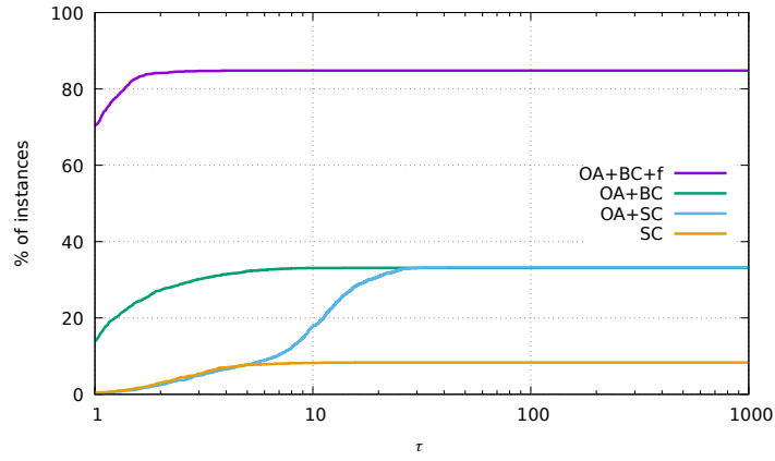
Figure 9: Performance profile comparing the four branch-and-cut algorithms for the p-matroid and p-matroid & confl classes.
