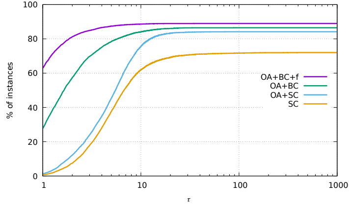
Figure 8: Performance profile comparing the four branch-and-cut algorithms for the kp and kp & confl classes.
