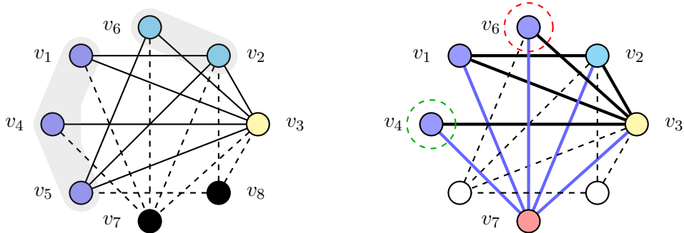
Figure 6: On the left, a (\kappa+1) -partite subproblem graph \hat{G} of a (\kappa+1) -partite branching node with \kappa=3 , together with a 4-coloring. The independent sets I_1 = \{v_1, v_4, v_5\} , I_2 = \{v_2, v_6\} and I_3 = \{v_3\} are the first 3 colours; the branching set B = \{v_7, v_8\} , in black, is the 4-th colour. On the right part, the (\kappa+1) -partite subproblem graph \hat{G} , with \kappa=2 , resulting from branching on the vertex v_7 in the reference node shown in the left part. Encircled vertices are filtered: v_6 (red) by FiltCOL and v_4 (green) by FiltSAT .
