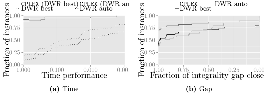
Figure 15: Performance profiles comparing DWR auto, DWR best and CPLEX
