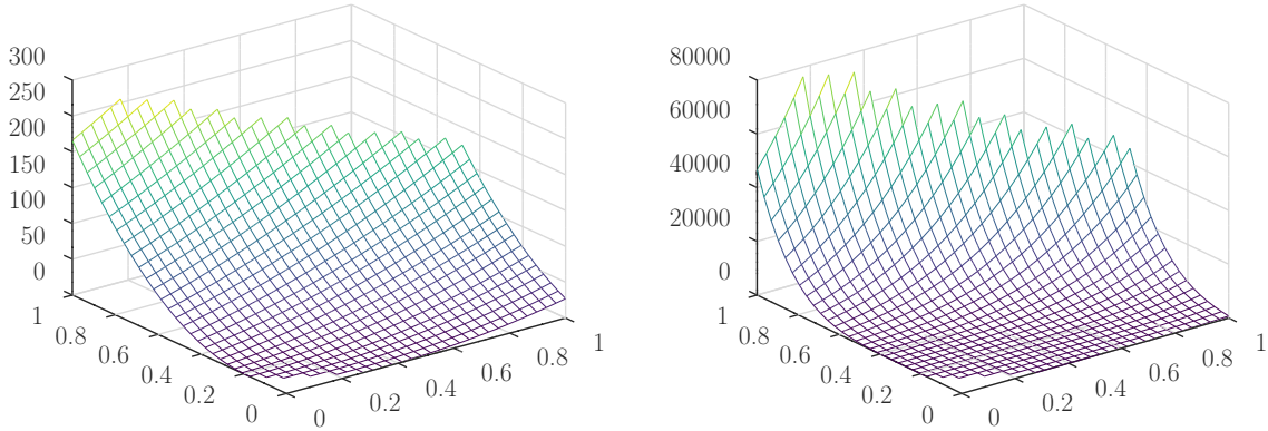
Figure 4: An illustration of the non-concave objective function of the (PHD-KP _\ell ) for an instance with n = 2 , p_1 = 4 , p_2 = 7 , \alpha = -1 , and c = 9 , subject to the constraint 5x_1 + 8x_2 \leq c , with \ell = 3 (left) and \ell = 6 (right). The objective function, which reads \frac{(4y_1 + 7y_2 + \alpha)^3}{y_1 + y_2} (left) and \frac{(4y_1 + 7y_2 + \alpha)^6}{y_1 + y_2} (right), is plotted only for the (x_1, x_2) \in [0, 1]^2 pairs which are feasible, i.e., which satisfy 5x_1 + 8x_2 \leq c and 4y_1 + 7y_2 - 1 > 0 .
