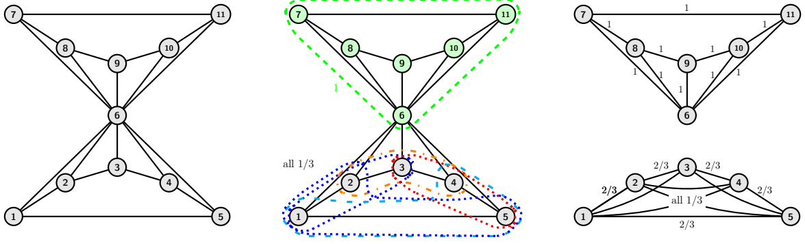
Figure 3: Partitioning with 2/3-quasi-cliques. (a) the graph G , (b) the fractional solution \lambda_{\{6,7,8,9,10,11\}} = 1 and \lambda_{\{1,2,3\}} = \lambda_{\{2,3,4\}} = \lambda_{\{3,4,5\}} = \lambda_{\{1,4,5\}} = \lambda_{\{1,2,5\}} = 1/3 , (c) the support graph in which the component P = \{1, 2, 3, 4, 5\} is no 2/3-quasi-clique, but P' = P \cup \{6\} = \{1, 2, 3, 4, 5, 6\} is a 2/3-quasi-clique
