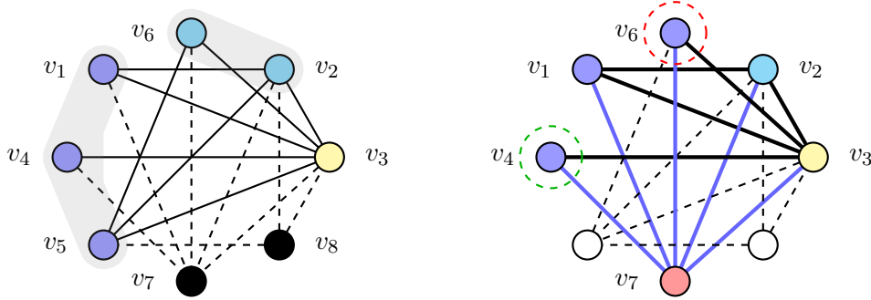
Figure 6: On the left, a (\kappa + 1) -partite subproblem graph \hat{G} of a (\kappa + 1) -partite branching node with \kappa = 3 , together with a 4-colouring. The independent sets I_1 = \{v_1, v_4, v_5\} , I_2 = \{v_2, v_6\} and I_3 = \{v_3\} are the first 3 colours; the branching set B = \{v_7, v_8\} , in black, is the 4-th colour. On the right part, the (\kappa + 1) -partite subproblem graph \hat{G} , with \kappa = 2 , resulting from branching on the vertex v_7 in the reference node shown in the left part. Encircled vertices are filtered: v_6 (red) by FiltCOL and v_4 (green) by FiltSAT .
