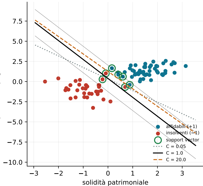
Soft margin: iperpiano, margine e support vector
