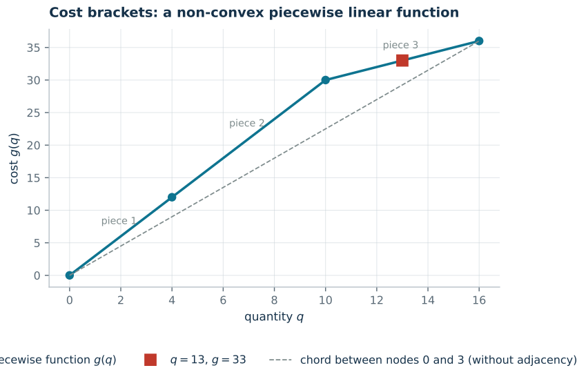
Figure 6.2: The piecewise function with a quantity discount. The dashed chord between the extreme nodes is what the formulation without adjacency can reach: it lies below the graph.
