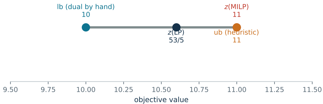
Figure 3.1: The four numbers of the protocol, on the assignment instance.
