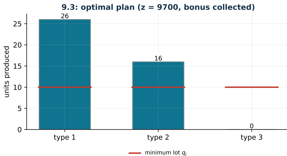
Figure 9.3: Optimal plan: units produced per type, with the minimum lot \bar{q}_j marked in red. Type 3 stays at zero.
