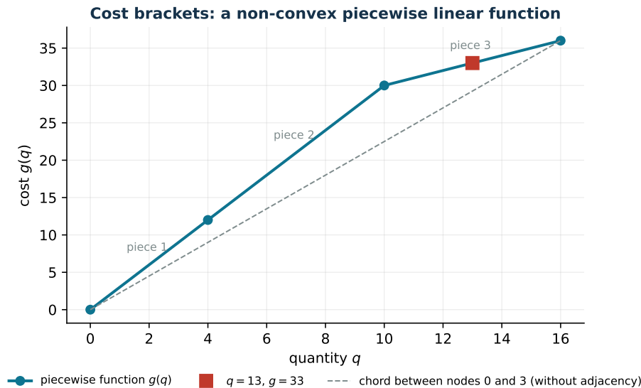
Figure 3.2: The piecewise function with a quantity discount. The dashed chord between the extreme nodes is what the formulation without adjacency can reach: it lies below the graph.
