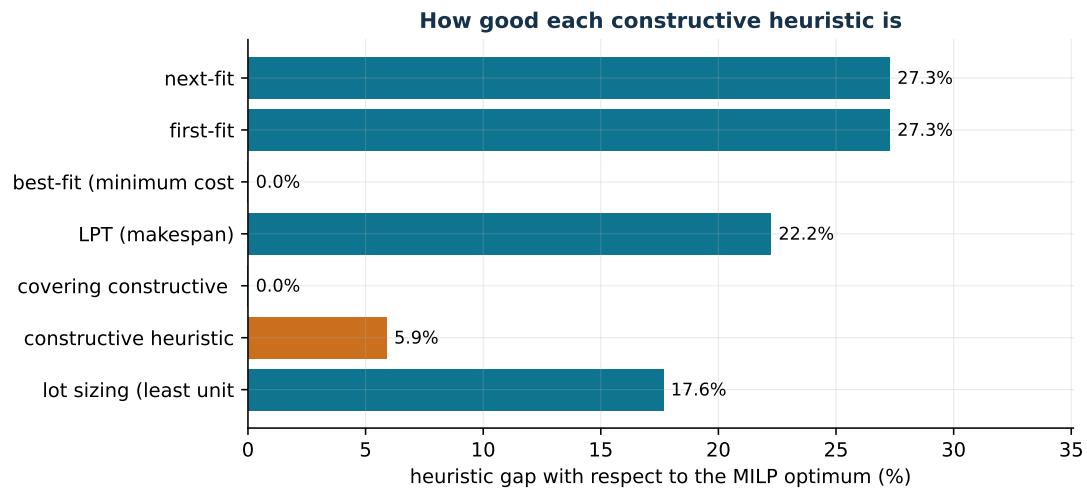
Figure 5.1: The gap of each heuristic with respect to the MILP optimum, on the minimal instances of this chapter. Teal for minimisation problems, orange for maximisation.
