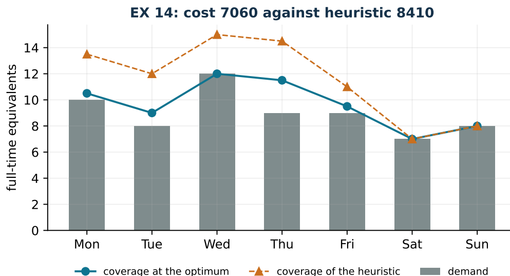
Figure 6.9: EX 14: daily demand and coverage, in the heuristic solution and in the optimal one.
