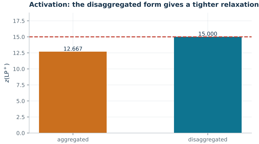
Figure 6.1: The relaxation of the two activation forms on the three-customer, two-site instance. The red line is the integer optimum.
