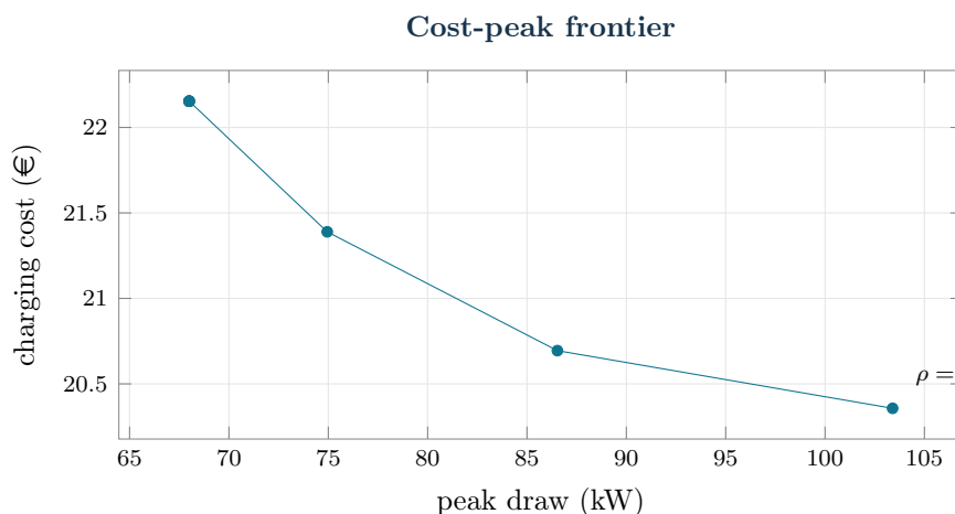
Figure 10.2: Cost-peak frontier obtained by varying the weight \rho of the peak in the objective: every point is an optimal charging strategy. Reducing the peak from 103 to 75 kW costs about one euro per night; the point \rho \geq 0.2 reaches the minimum possible peak (68 kW) at the lowest cost that allows it.
