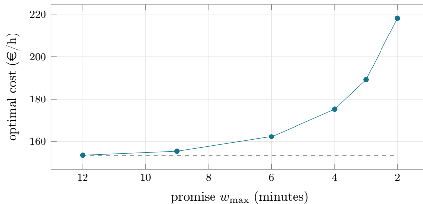
Figure 11.2: Optimal cost as a function of the service promise w_{\max} (reversed axis: towards the right the promise becomes more ambitious). The dashed line is the cost without any promise: up to 12 minutes the promise is almost free, below 4 minutes every additional minute cut costs explosively.
