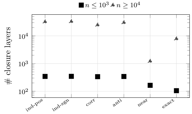
Figure 4: Median number of closure layers per coefficient family, reported separately for the small and the large sizes. Instances: mixed-forest , all four densities, n \in \{100, \dots, 1\,000\} (2400 instances) and n \in \{10\,000, \dots, 100\,000\} (2400 instances). Observations: how much parametric structure each family creates – the single most useful fact for reading absolute times, since the work of every algorithm scales with the number of breakpoints. At n \geq 10^4 the median layer count ranges from 1222 ( near-ties ) to 33183 ( independent-signed ), a factor of 27 at equal size. This is why the tie-stressing families are the fastest in every timing table below, which would otherwise look counter-intuitive.
