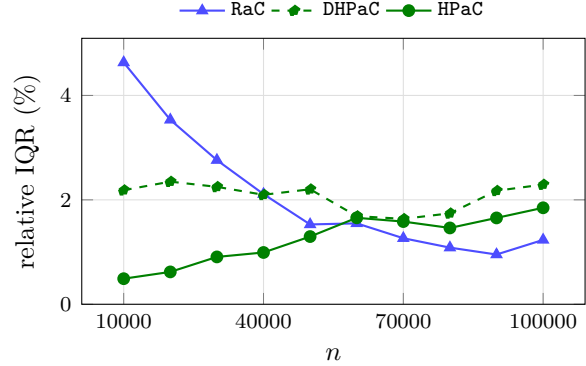
Figure 36: Median relative IQR of the timing, in percent, per size: for each instance, the IQR over its repetitions divided by its own median time, then the median of that over instances. Instances: mixed-forest , n \in \{10\,000, \dots, 100\,000\} , 240 instances per size, 3 repetitions each. Observations: 0.5% to 1.8% for HPaC, 1.6% to 2.3% for DHPaC, and 4.6% falling to 1.2% for RaC – the longer a run, the smaller its relative noise, which is why the largest sizes are the quietest. This is the number that says how much of a reported difference is signal: every ratio in this report is at least an order of magnitude larger than the measurement noise it rests on. The single exception is the near-tie 0.91 against 1 at n = 100 in Section 8.1, which is for that reason reported as a near-tie and not as an advantage.
