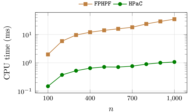
Figure 34: Median CPU time in milliseconds of HPaC and of FPHPF , per size, both solving each instance from scratch; “ratio” is the median over the instances of the paired ratio FPHPF / HPaC . Instances: mixed-forest , n \in \{100, 200, \dots, 1\,000\} , 240 per size, 2 400 in total; 11 repetitions per side. Observations: the two methods return the same partition and the same breakpoints on all 2 400 instances, and HPaC is faster on every one of them; the median paired ratio grows from 9.2 at n = 100 to 27.6 at n = 1\,000 , overall median 19.5 (p10 7.1, p90 75.7). The ratio is largest on sparse forests ( \varrho = 0.3 : median 52.5, many small trees and hence many layers) and smallest on the two tie-stressing families ( exact-ties 12.1, near-ties 14.7, fewer layers to separate). Scope: forests, whereas FPHPF solves a strictly more general problem on arbitrary precedence graphs; recall that on a forest its bound reads \mathcal{O}(n^2 \log n) (Table 1).
