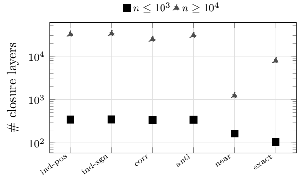
Figure 4: Median number of closure layers per coefficient family, reported separately for the small and the large sizes. Instances: mixed-forest , all four densities, n \in \{100, \dots, 1\,000\} (2 400 instances) and n \in \{10\,000, \dots, 100\,000\} (2 400 instances). Observations: how much parametric structure each family creates – the single most useful fact for reading absolute times, since the work of every algorithm scales with the number of breakpoints. At n \geq 10^4 the median layer count ranges from 1 222 ( near-ties ) to 33 183 ( independent-signed ), a factor of 27 at equal size. This is why the tie-stressing families are the fastest in every timing table below, which would otherwise look counter-intuitive.
