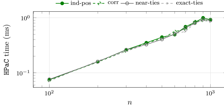
Figure 37: Median CPU time of HPaC in milliseconds, one column per coefficient family and one row per size. Instances: mixed-forest , n \in \{100, \dots, 1000\} , all four densities, 40 instances per cell. The plot shows four of the six families, the table all six. Observations: at these sizes all times are sub-millisecond and the six families are indistinguishable at the reported resolution – the largest gap at any size is one tenth of a millisecond, i.e. the last digit. The family effect exists but needs n \geq 10^4 to be measurable (Fig. 39); this table is here to show that it is not measurable below that, so no conclusion in Section 8.1 rests on it.
