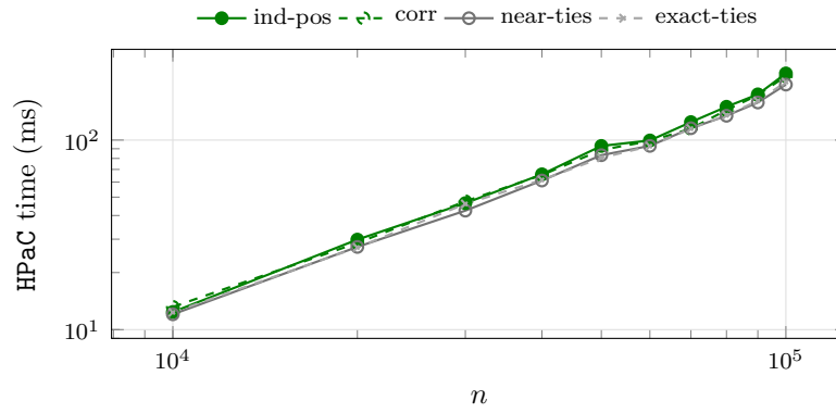
Figure 39: Median CPU time of HPaC in milliseconds, one column per coefficient family and one row per size. Instances: mixed-forest , n \in \{10\,000, \dots, 100\,000\} , all four densities, 40 instances per cell. The plot shows four of the six families, the table all six. Observations: here the family effect is measurable and consistent – the two tie-stressing families ( near-ties , exact-ties ) occupy the two fastest columns at 9 of the 10 sizes, and anti-correlated or independent-signed the slowest – with a spread between fastest and slowest family of 8–17% that neither grows nor shrinks with n . Compare Fig. 4: near-ties produces 27\times fewer closure layers than independent-signed at these sizes, yet costs only about 10% less time – so the per-layer cost is far from constant, and most of HPaC’s work at n = 10^5 is proportional to n (building and rebuilding the heaps) rather than to the number of breakpoints.
