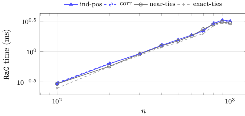
Figure 38: Median CPU time of RaC in milliseconds, one column per coefficient family and one row per size. Instances: mixed-forest , n \in \{100, \dots, 1000\} , all four densities, 40 instances per cell. The plot shows four of the six families, the table all six. Observations: the same picture as Fig. 37 a factor of three higher, with the families within 0.5 ms of each other at n = 1000 . Every family shows the same dip from n = 900 to n = 1000 (3.5 to 3.1 ms for anti-correlated ), and so does HPaC, while the number of closure layers keeps growing (470 to 528) and PaC keeps growing with it. We attribute the two elevated sizes to memory-bandwidth contention between the parallel lanes of the sweep (Section 4), which touches the two memory-bound algorithms and not the scan-based one; the effect is \approx 10\% , an order of magnitude below every ratio reported in this document, and it is visible only in this per-cell breakdown.
