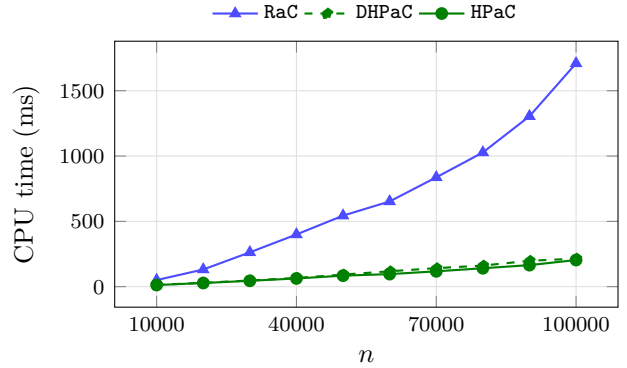
Figure 12: Median CPU time in milliseconds of HPaC, DHPaC and RaC, per size. Instances: mixed-forest , n \in \{10\,000, 20\,000, \dots, 100\,000\} , 240 instances per size (four densities \times six families \times ten seeds), 3 repetitions each. Observations: HPaC computes the full parametric solution on 10^5 vertices in about 0.2s; DHPaC stays within 25% of it at every size and is marginally faster at n = 10^5 , so the primal/dual choice is immaterial at scale; RaC is above both throughout, by a factor that grows with n (Fig. 13).
