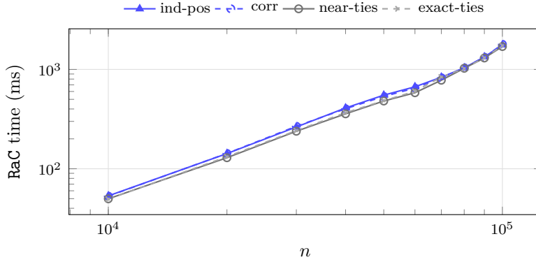
Figure 40: Median CPU time of RaC in milliseconds, one column per coefficient family and one row per size. Instances: mixed-forest , n \in \{10\,000, \dots, 100\,000\} , all four densities, 40 instances per cell. The plot shows four of the six families, the table all six. Observations: the family spread is 4–10%, i.e. narrower than HPaC’s, and the ordering is the same, which is why the paired ratio of Fig. 17 is flat: the two algorithms react to the coefficients in the same way. RaC’s growth over this range is the steepest of any algorithm here – a factor 33 (53 to 1 766 ms) for a 10\times increase in n , against a factor 17 for HPaC – which is consistent with its being the only algorithm whose space is \mathcal{O}(n \log n) : past a few tens of thousands of vertices its top-tree structures no longer fit in cache and every contraction round pays main-memory latency. We report this as an interpretation, not as a measurement: we did not instrument cache misses.
