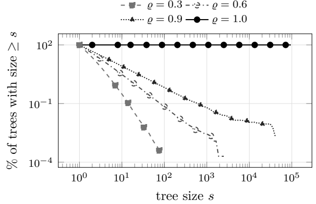
Figure 3: Distribution of the tree size: for each size s , the percentage of trees with at least s vertices, one curve and one column per density, on the 40 mixed-forest instances with n = 100\,000 (10 per density); the table lists the same distribution at selected sizes. The distribution is heavy-tailed at every density below 1: at \varrho = 0.3 , 77% of the trees are single vertices and only 0.3% reach 10 vertices, yet the largest reaches 96. At \varrho = 0.9 the tail detaches completely – 30% of trees have \geq 3 vertices and one tree of \approx 4 \cdot 10^4 vertices appears, four orders of magnitude above the median. This is the percolation-like transition that Fig. 14 sees as a timing effect: what changes between \varrho = 0.6 and \varrho = 0.9 is not the number of trees (it falls smoothly) but the emergence of one giant tree, and RaC’s per-component overhead is paid on the count of trees while its contraction rounds are amortized over the giant one.
