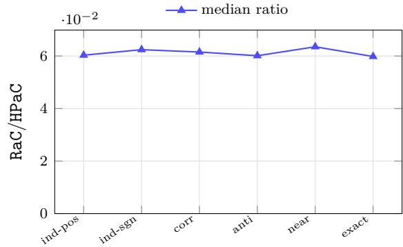
Figure 21: Stars by family: absolute times (left) and the paired ratio RaC/HPaC (right), between 0.060 and 0.064 in all six. The inversion is purely topological: no coefficient family produces it and none removes it.
