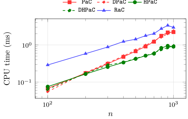
Figure 5: All five algorithms on mixed-forest instances, n \in \{100, 200, \dots, 1000\} (240 instances per size). The two families are indistinguishable up to n \approx 300 and the heap pays off from n \approx 400 on; each dual tracks its primal throughout, which is why the manuscript reports only the primals. PaC re-scans every candidate ratio at every iteration, while HPaC extracts the maximum in logarithmic time and refreshes only the candidates touched by the last peel or contraction.
