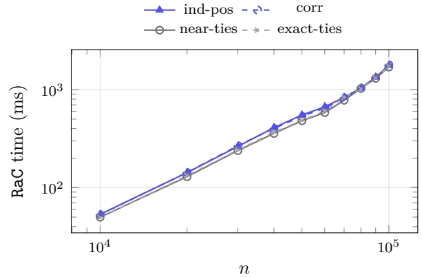
Figure 37: RaC on mixed-forest instances, n \geq 10000 .
