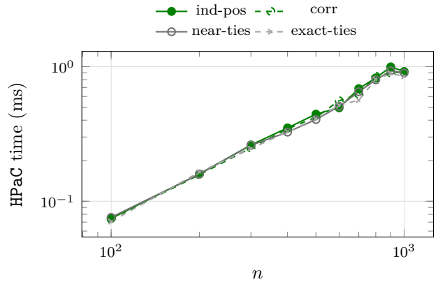
Figure 34: HPaC on mixed-forest instances, n \leq 1000 .
