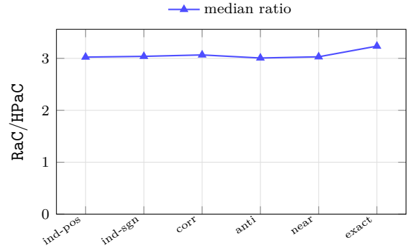
Figure 29: For completeness, RaC against the general HPaC on the same oriented instances, by family (out-forests behave the same). RaC loses ground as n grows here too, from about 2.8\times at n \leq 1000 to 12.8\times at n = 10^5 .
