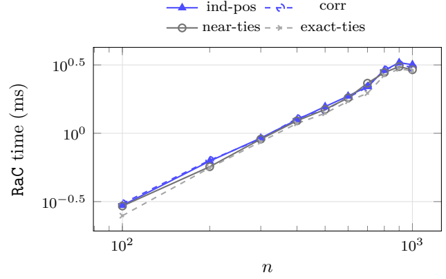
Figure 35: RaC on mixed-forest instances, n \leq 1000 .
