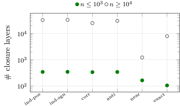
Figure 2: How much parametric structure each coefficient family creates. This is the single most useful fact for reading absolute times, since the work of every algorithm scales with the number of breakpoints: at n \geq 10^4 the median layer count ranges from 1 222 ( near-ties ) to 33 183 ( independent-signed ), a factor of 27 at equal size. It also explains why the tie-stressing families are the fastest in every timing table below, which would otherwise look counter-intuitive.
