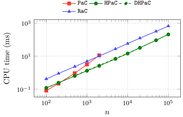
Figure 18: binary-mixed instances (60 per size): median RaC/HPaC between 3.2 and 3.9 over the whole range – lower than on paths, since a balanced tree gives RaC's contraction rounds more to work with.
