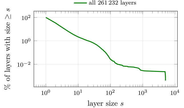
Figure 4: Size of the closure layers, measured on 60 instances at n = 10\,000 (261 232 layers). The distribution is extremely skewed : overall median 1, mean 2.3, and two thirds of all layers are singletons – yet the largest single layer holds 5 077 vertices, half the graph. So a parametric solution is typically a long chain of one-vertex layers plus a handful of very large blocks, and an algorithm’s cost per layer matters more than its cost per vertex. Two group-level facts stand out. The tie-stressing families behave completely differently from the others: near-ties has median layer size 7 and no singletons at all (by construction, vertices share thresholds), against median 1 and 73–75% singletons for the independent families – which is the mechanism behind their much smaller layer counts (Fig. 2). And density compresses the largest layer by an order of magnitude: on sparse random forests the biggest layer holds 563 vertices, against \approx 5\,000 once the graph is a single tree, because a layer cannot straddle components.
