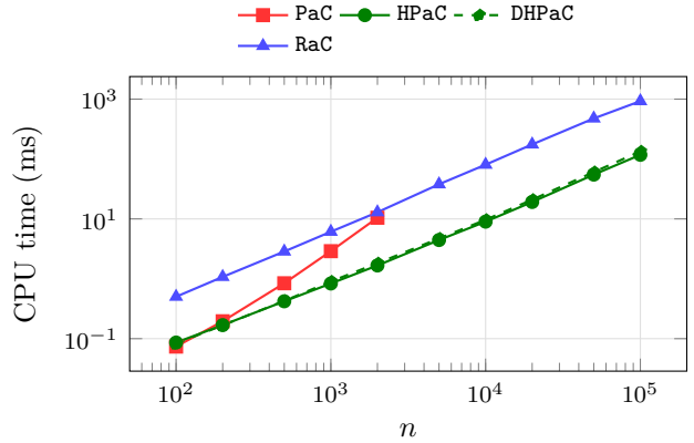
Figure 16: path-mixed instances (60 per size). These behave like random forests: median RaC/HPaC between 5.8 and 9.0 over the whole range, and PaC left far behind by n = 10^4 , as its \mathcal{O}(n^2) bound predicts.
