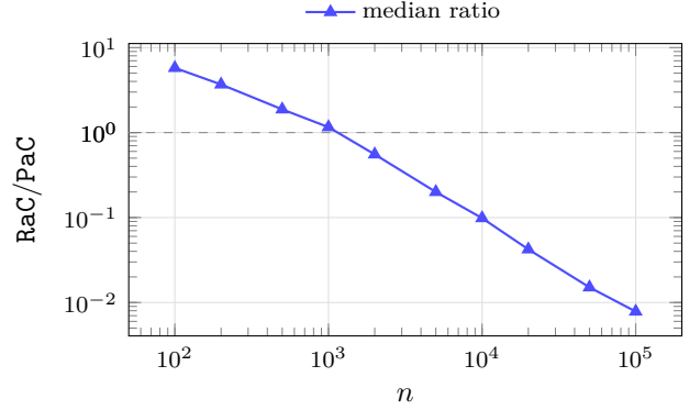
Figure 22: Stars, RaC against PaC: the comparison between the two algorithms that are not penalized by a candidate structure on a hub, and therefore the one that isolates the asymptotic difference. The crossover sits between n = 1\,000 and n = 2\,000 ; by n = 10^5 RaC is 130\times faster. Dashed line marks parity.
