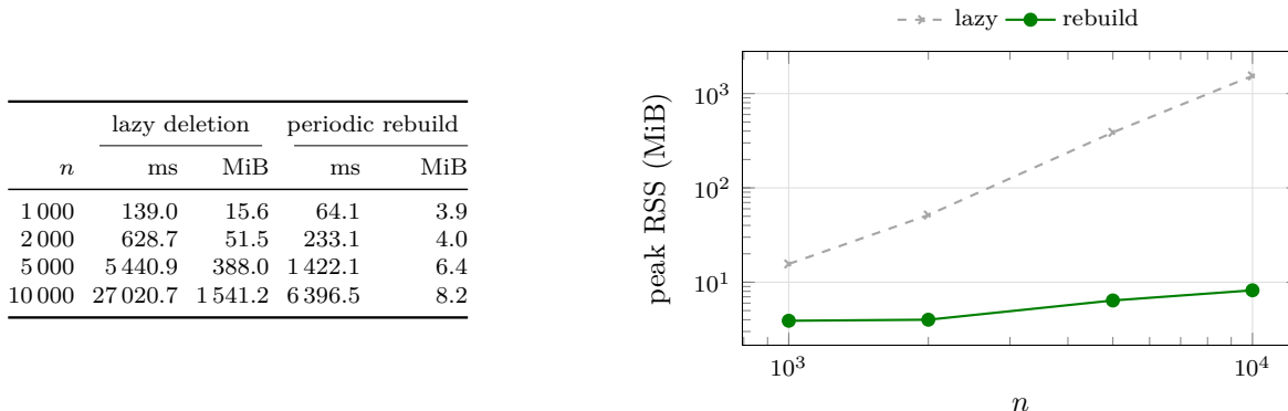
Figure 30: The two policies on star-mixed instances ( independent-positive , seed 0, one repetition; single-algorithm invocations, the only regime in which peak RSS is attributable to one algorithm). The lazy heap’s memory grows by a factor of 100 when n grows by 10 – quadratic, as predicted – reaching 1.5 GiB at n = 10^4 where the rebuild policy uses 8 MiB; extrapolating, the lazy policy exhausts an 8 GiB ceiling by n \approx 20\,000 . The rebuild policy is also \approx 4\times faster here (and \approx 2\times on large random forests), with bit-identical output on every instance tested. For reference, PaC, which maintains no candidate structure, peaks at 5.6 MiB at n = 10^4 . The practical lesson: on this problem the choice of data structure inside one algorithm is worth as much as the choice between algorithms.
