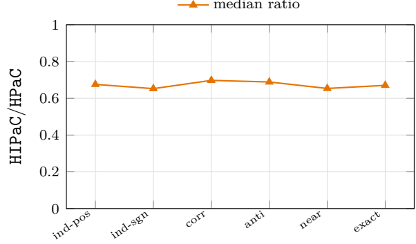
Figure 31: Median of the paired per-instance ratio HIPaC/HPaC, per coefficient family, with the number of paired instances and the IQR. Instances: in-forest , all sizes and densities pooled, 800 instances per family. Observations: the ratio lies between 0.65 and 0.70 in all six families, a 7% spread – against the factor 6 across densities of Fig. 30. There is no family in which the advantage of the specialization disappears, and none in which it is much larger: as everywhere else in this report, the coefficients set the amount of work and the topology sets who wins.
