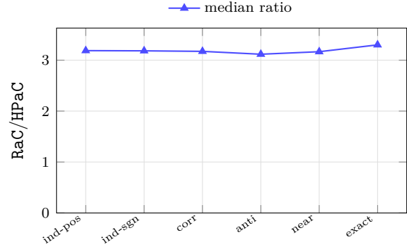
Figure 11: Median of the paired per-instance ratio \text{RaC}/\text{HPaC} , per coefficient family, with the number of paired instances and the IQR. Instances: mixed-forest , n \in \{100, \dots, 1\,000\} and all four densities pooled, 400 instances per family. Observations: the ratio is flat at 3.1–3.3 across all six families – at these sizes the coefficient family changes how much work there is, not which algorithm does it faster.
