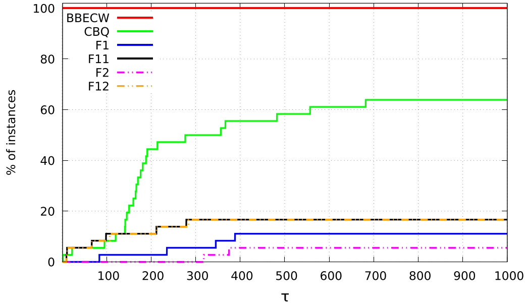
Fig. 6. Performance profile on the DIMACS instances.
