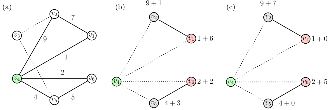
Fig. 3. Illustration of the computation of the upper bound UB(P, \mathcal{S}, \tilde{\rho}) . (a) The original graph, with an incumbent solution C = \{v_4\} of value 0, highlighted in green, and candidate vertex set \hat{V} = \{v_1, v_2, v_5, v_6\} . We assume P = \hat{V} . (b) The number associated with each vertex u is equal to \hat{w}_u , i.e., to the sum of w_u and \sum_{e \in \delta(u, P)} \tilde{\rho}_e^u (the two terms are reported with a '+' symbol between them). The collection \mathcal{S} consists of two independent sets I_1 = \{v_1, v_6\} (in red) and I_2 = \{v_2, v_5\} (in gray), with \tilde{\pi}_{I_1} = \max\{7, 4\} = 7 , \tilde{\pi}_{I_2} = \max\{10, 7\} = 10 . The upper bound UB(P, \mathcal{S}, \tilde{\rho}) is equal to \tilde{\pi}_{I_1} + \tilde{\pi}_{I_2} = 17 (also equal to the optimal solution value). (c) A different choice of \tilde{\rho} gives the upper bound UB(P, \mathcal{S}, \tilde{\rho}) = \tilde{\pi}_{I_1} + \tilde{\pi}_{I_2} = 7 + 16 = 23 . (For interpretation of the references to color in this figure legend, the reader is referred to the web version of this article.)
