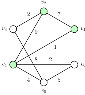
Fig. 1. A graph G with |V| = 6 vertices and |E| = 8 edges. The clique C = \{v_1, v_2, v_4\} (whose vertices are highlighted in green) is the (unique) maximum edge-weighted clique that G contains. The edge-weighted clique number of G is \omega_c(G) = c(C) = 17 . (For interpretation of the references to color in this figure legend, the reader is referred to the web version of this article.)
