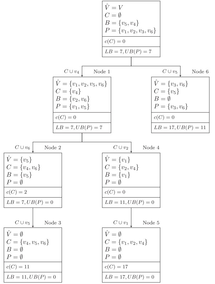
Fig. 4. Branch-and-bound tree produced by the BBEWC algorithm for the graph of Fig. 1.
