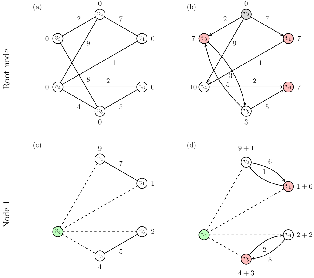
Fig. 5. Illustration of the creation of the branching and pruned sets B and P for the root node (above) and node 1 (below) of the branch-and-bound tree of Fig. 4. The subfigures parts (a) and (c) report \hat{G} of the node with the corresponding vertex weights w_u . The subfigures parts (b) and (d) report the independent sets in \mathcal{S} (in red and gray), the values of \hat{w}_u , those of \hat{p}_e^u , and the partial clique C = \{v_4\} (in green). For every e = \{u, v\} \in \hat{E} , an arc going from u to v represents the variable \hat{p}_e^u (only if strictly positive). The number associated with each vertex u is equal to \hat{w}_u , written as the sum of w_u and \sum_{e \in \delta(u, \hat{V})} \hat{p}_e^u . (For interpretation of the references to color in this figure legend, the reader is referred to the web version of this article.)
