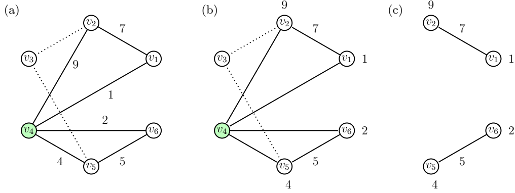
Fig. 2. Illustration of the vertex weight induced by C on the nodes u \in \hat{V} . (a) The original graph, with an incumbent solution C = \{v_4\} of value 0, highlighted in green, and candidate vertex set \hat{V} = \{v_1, v_2, v_3, v_4, v_5, v_6\} . (b) The original graph with a number associated with each vertex u equal to w_u as defined in Eq. (2). Notice that the edge weight of each edge e \in E[\hat{V}] is unchanged. (c) The edge and vertex-weighted graph \hat{G} = (\hat{V}, \hat{E}) , with the corresponding vertex weight induced by C and the original edge weight on its edges. (For interpretation of the references to color in this figure, the reader is referred to the web version of this article.)
