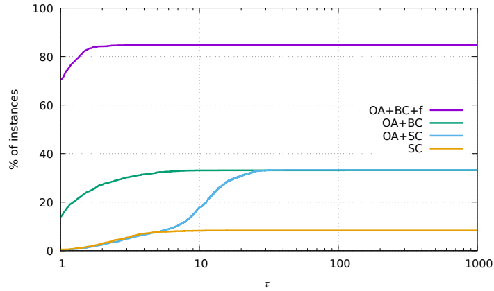
Figure 9: Performance profile comparing the four branch-and-cut algorithms for the p-matroid and p-matroid & confl classes. fig:performance_profile_3
