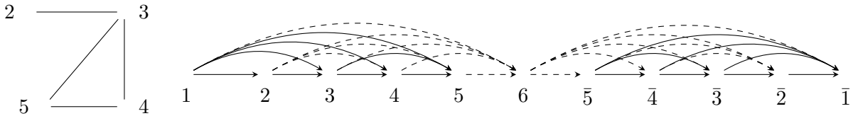
Figure 4: Transformation from CLIQUE problem into the BCSP on the DAG G^f .
