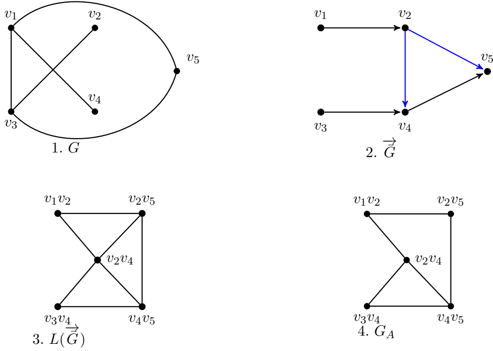
Figure 1: Transformation from a graph G to G_A
