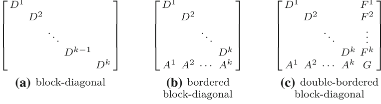
Fig. 1 Matrix forms
