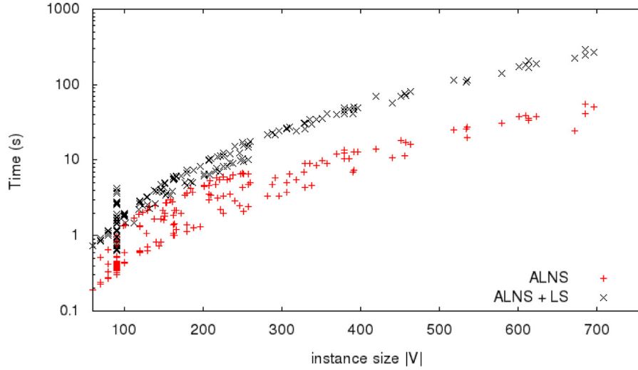
Fig. 5. Running time of heuristics, versus instance size (measured in number of vertices of the graph).
