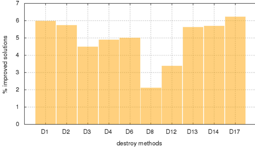
Fig. 3. Percentage of times in which each destroy method has produced an improving solution (together with some repair method).
