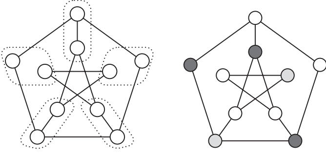
Fig. 1. Example: (left) a graph G and a partition of its vertices in 5 subsets ( k = 5 ); (right) a feasible Partition Coloring of G with two colors (gray and black).
