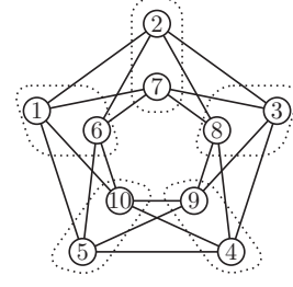
Fig. 2. Example: A graph G of 10 vertices and a partition of its vertices in 5 subsets ( k = 5 ).
