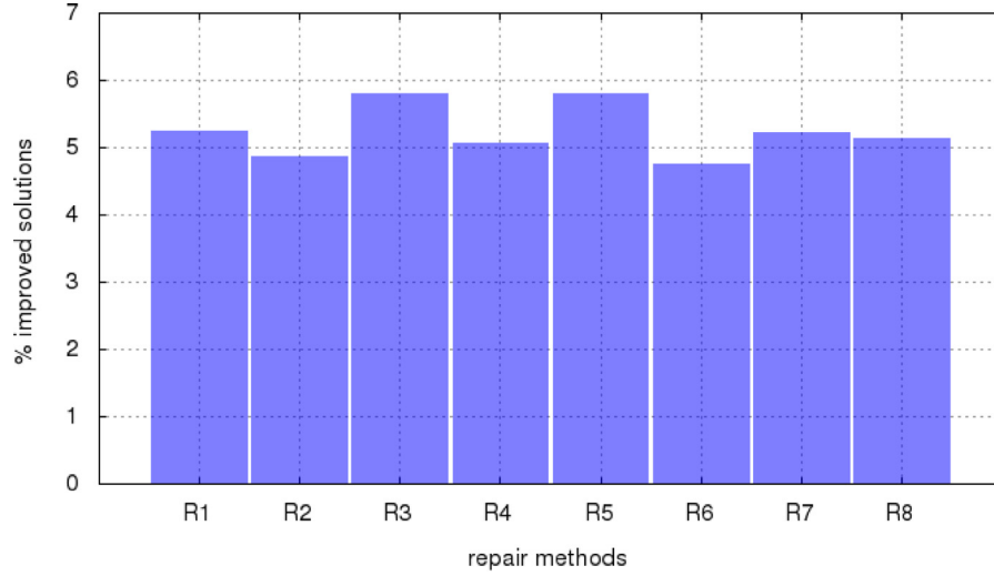
Fig. 4. Percentage of times in which each repair method has produced an improving solution (together with some destroy method).
